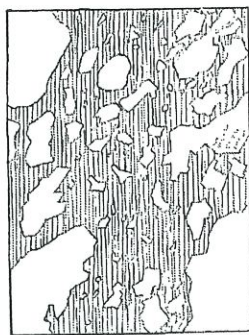
FIGURE 1—Section of brecciated ore from Murray Mine.
