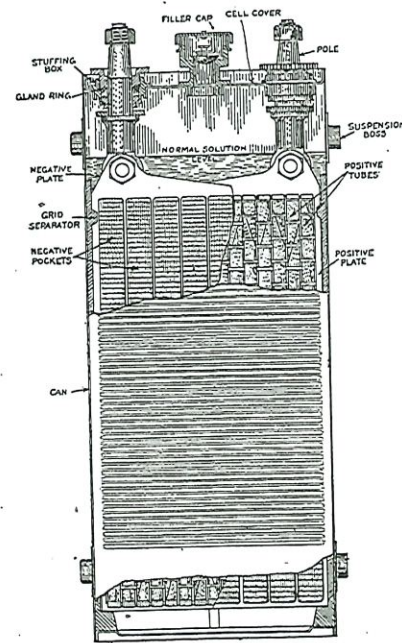
EDISON CELL IN SECTION
