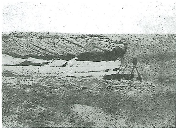
Fig. 1.—Cross-bedding in sandstone near Taylorton.
