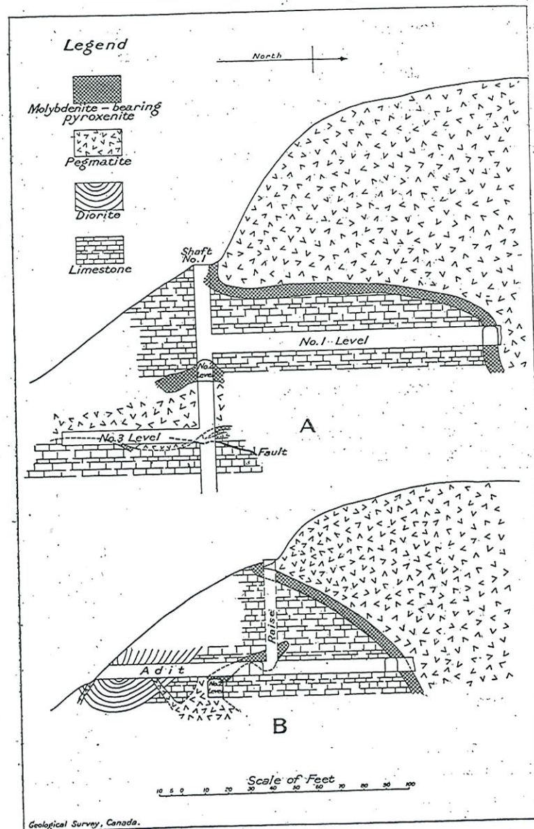
Fig. 3—North-South cross sections showing contact relationships of molybdenite ore-masses, Renfrew Molybdenum Mines, Ltd., lots 8 and 9, con. XI, Brougham tp., Renfrew county, Ontario.
