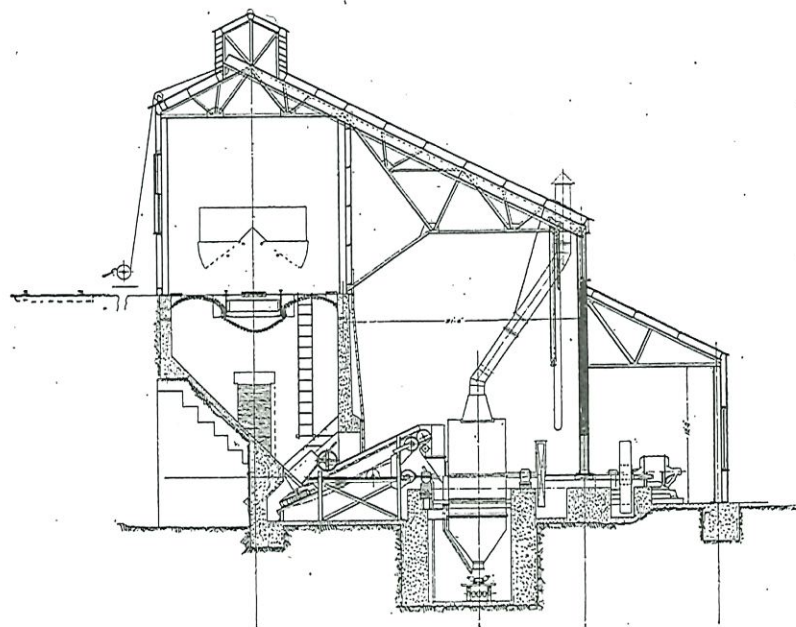
Figure 24.—Cross-section of crushing house, reverberatory plant.
