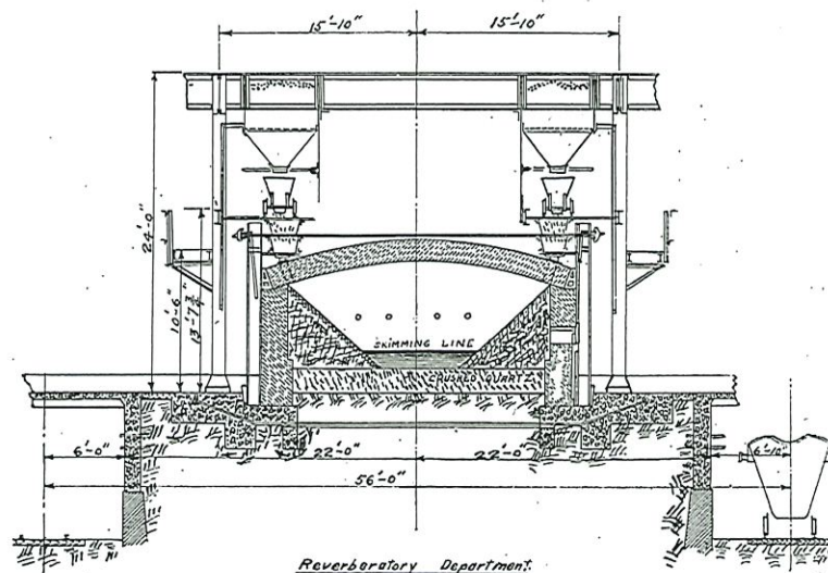
Figure 22.—Cross section of reverberatory furnace.
