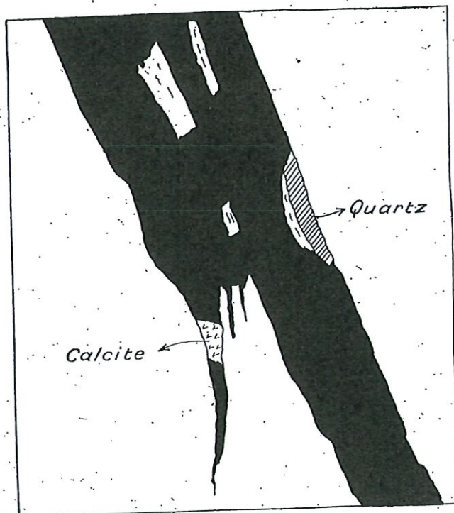
Fig. 47—Character of ore body at Victoria mine at narrow end of a lens, eleventh level. Black represents sulphides; white represents greenstone. Width of face 12 inches. The calcite, quartz and sulphides appear to have been deposited during the same period of mineralization.
