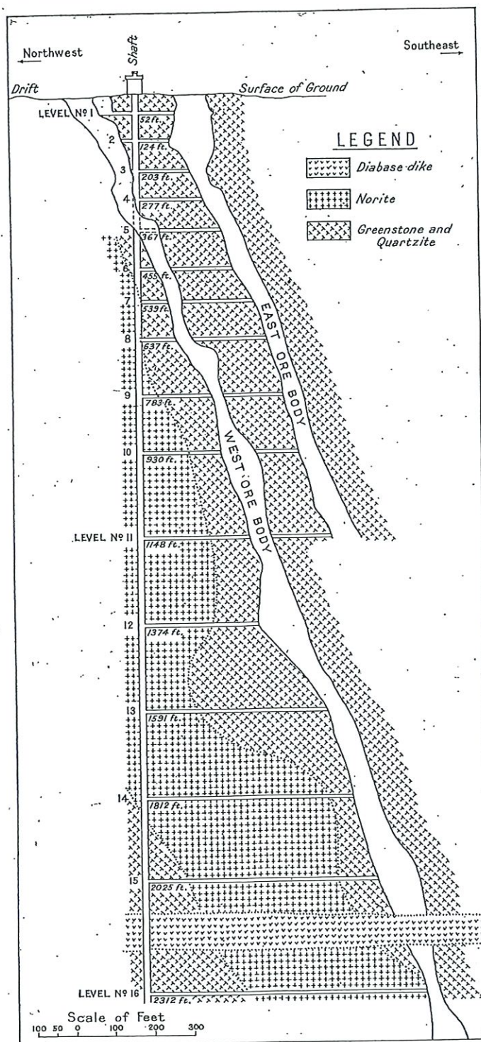
Fig. 44—Cross-section through Victoria ore bodies, Sudbury area, Ontario. At the time this Report was written the Victoria mine was the deepest in the Sudbury area, the west ore body having been worked to a vertical depth of 2,312 feet, and the shaft having been sunk to a depth of 2,618 feet.
