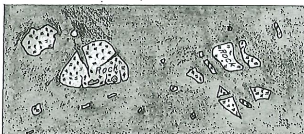
Fig. 6.—Character of ore at Creighton mine, Sudbury area, Ontario, ninth level, 15 feet from footwall. Greenstone boulders and fragments enclosed in sulphides (shaded area). Width of face 8 feet.
