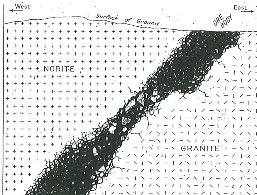
Fig. 21—Ideal cross-section through Creighton ore body, from the surface to the proposed eighteenth level, showing the nature of the deposit. Black represents ore. The norite is "spotted" with "blebs" of ore, about the size of peas, for 2,000 feet beyond the ore body. This "spotted" norite is not indicated in the drawing except along the edges. The granite is also "spotted" with ore, but to a much less extent than the norite. While the commercial ore body occurs about at the contact of the norite and granite, nevertheless the commercial ore body is found largely in the granite footwall—not in the norite.
