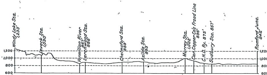
Fig. 3—Section from Romford Junction, near Sudbury, Ontario, to Windy lake, along the main line of the Canadian Pacific Railway. This section crosses the Sudbury basin and shows the elevations above sea level along the railway track. Horizontal scale 8 miles equals 1 inch; vertical scale 1,600 feet equals 1 inch.
