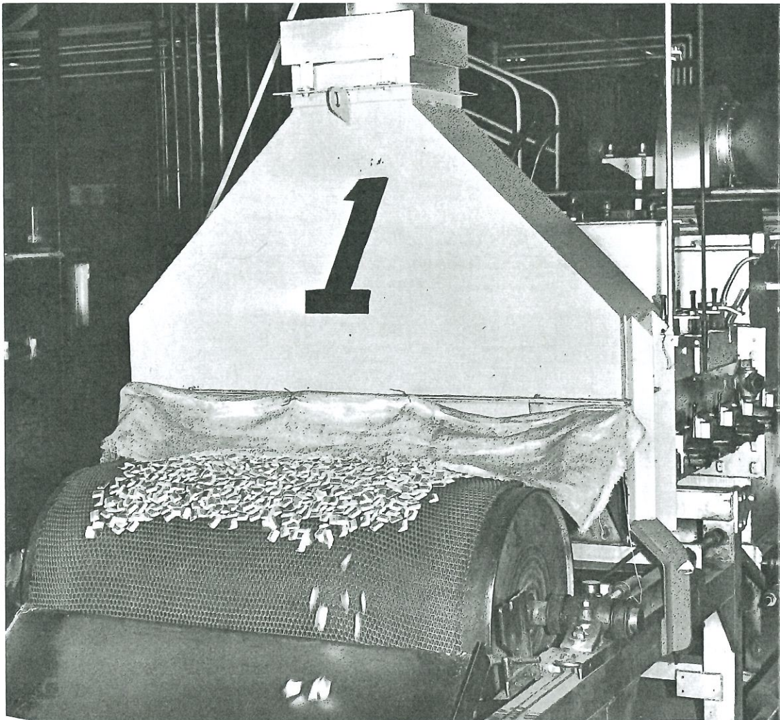
FIGURE 28. Sintering furnace for nickel briquettes, Fort Saskatchewan refinery.
