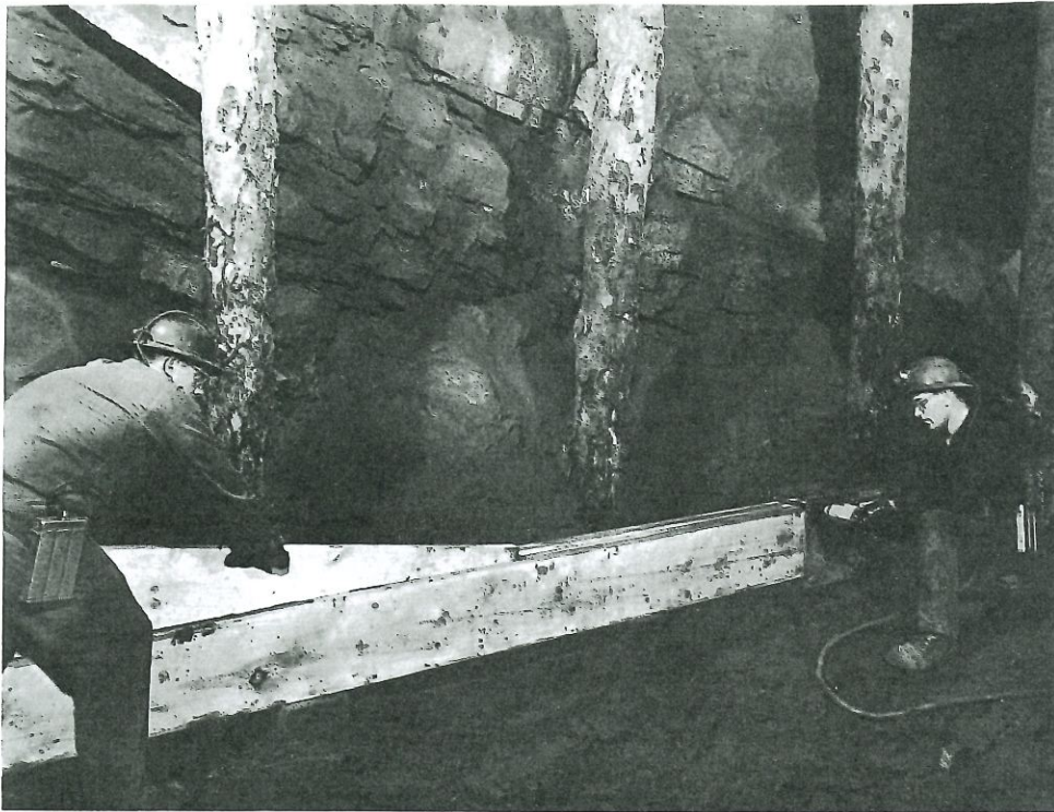
FIGURE 11. Constructing a laminated stringer in undercut-and-fill stope.
