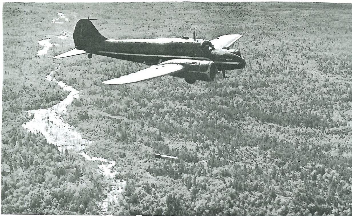
FIGURE 5. Airborne geophysical survey, magnetometer suspended beneath aircraft.
