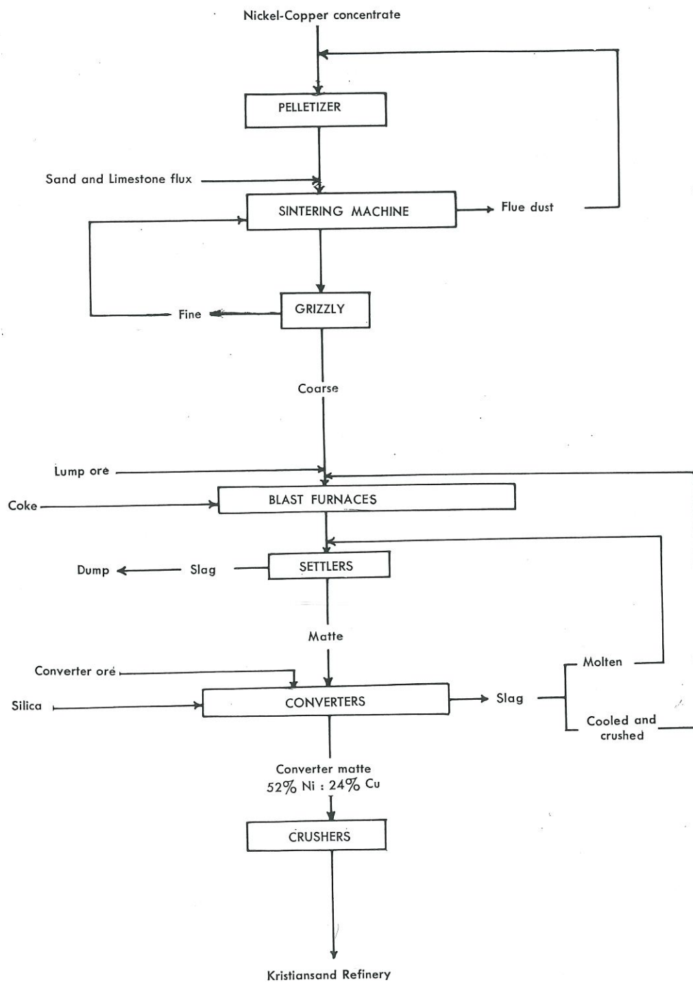
FIGURE 22. Generalized flowsheet, Falconbridge smelter.
