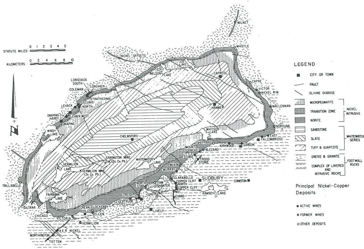
FIGURE 44. Geological map of the Sudbury district.
