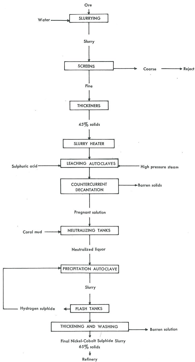
FIGURE 32. Generalized flowsheet, sulphuric acid leach process.
