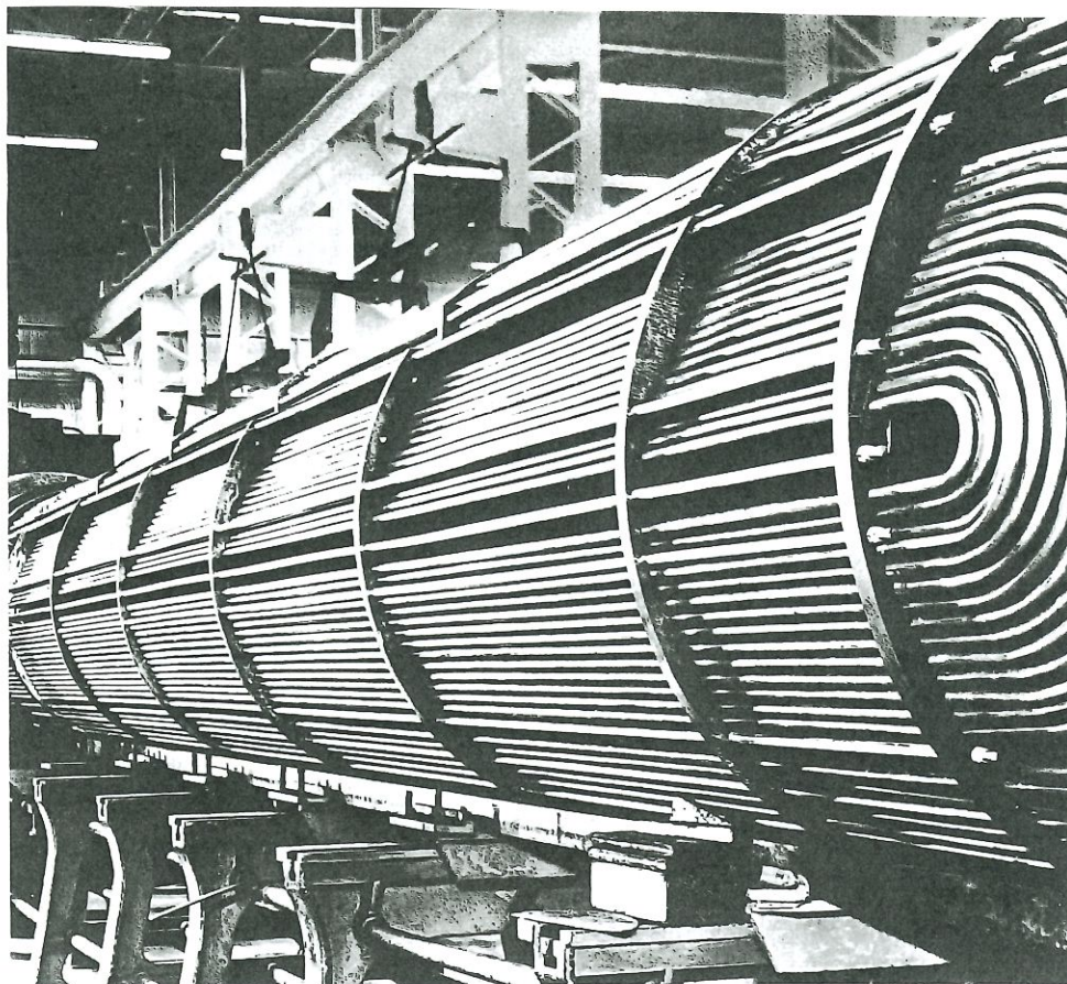
FIGURE 38. Copper-nickel alloy tubing for sea water desalinization plant.
