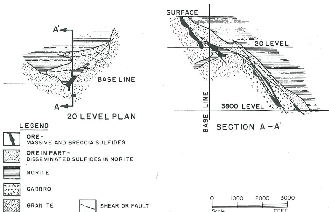
FIGURE 48. Generalized geological plan and section, Creighton mine.
