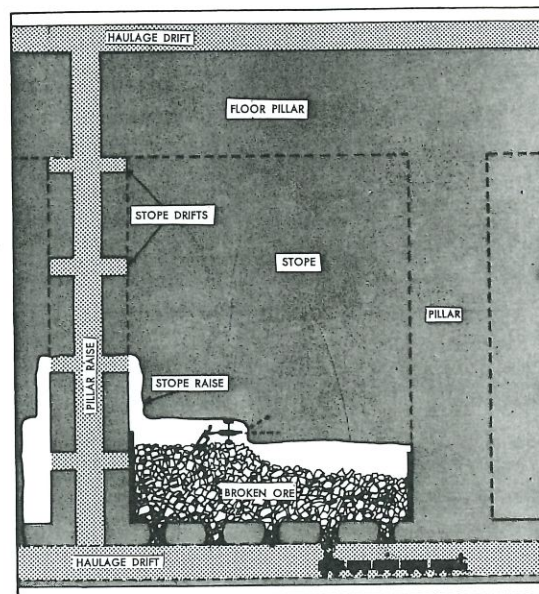
FIGURE 7. Generalized section of longitudinal shrinkage stope.
