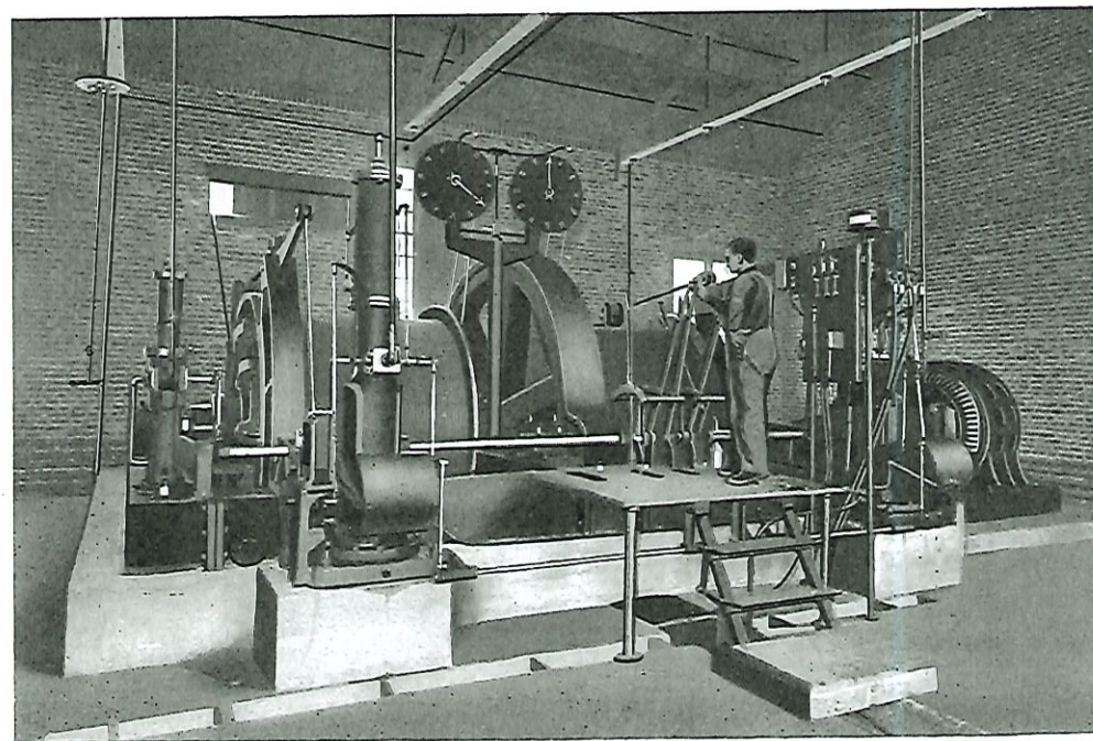
WORTHINGTON MINE. ELECTRICAL HOIST.
