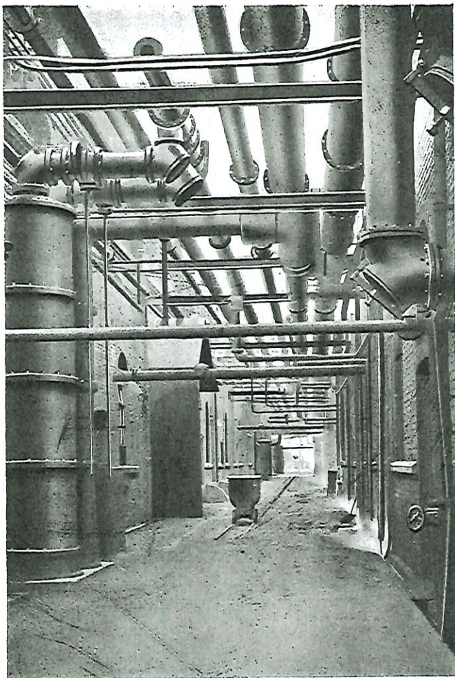
NICKEL REFINING WORKS. PIPE RANGE IN ROADWAY.
