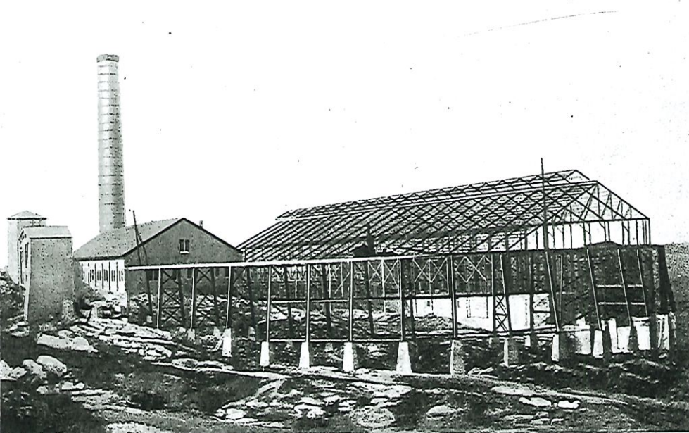
CONISTON SMELTER IN COURSE OF ERECTION. OCTOBER, 1912.
