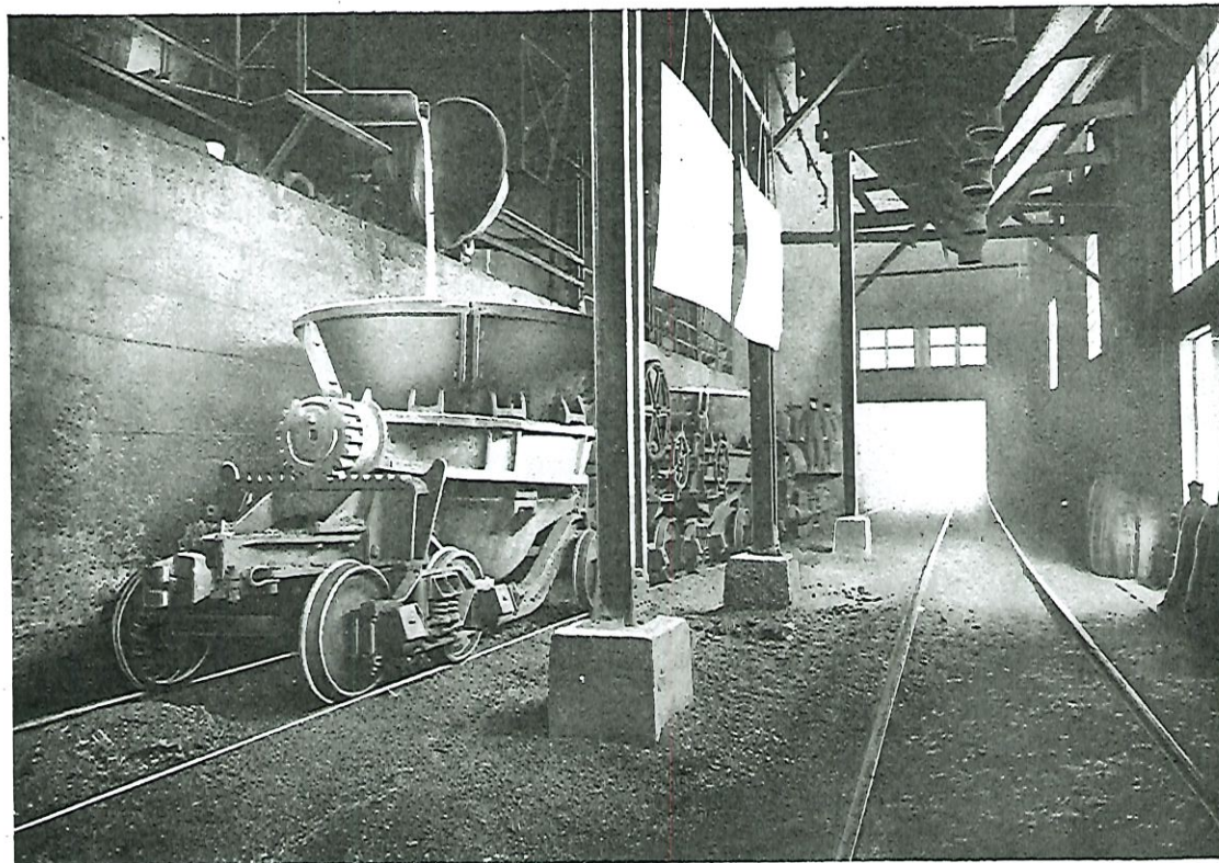
CONISTON PLANT. TRAIN OF CARS BEING CONVEYED BY LOCO. TO SLAG DUMP.
