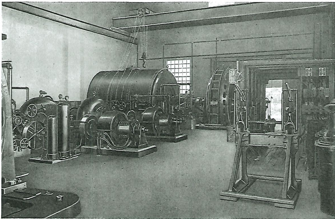
WABAGESHIK POWER PLANT. INTERIOR VIEW SHOWING NO. 1 UNIT.
