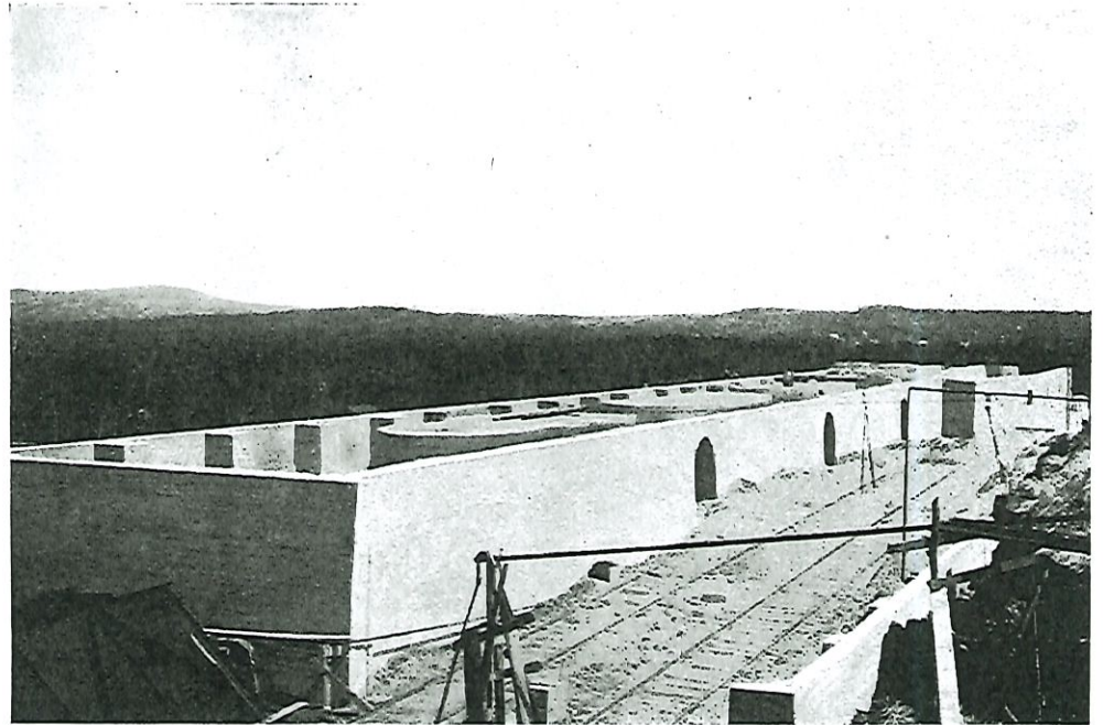
A PART OF THE FOUNDATIONS OF CONISTON SMELTER. JUNE, 1912.
