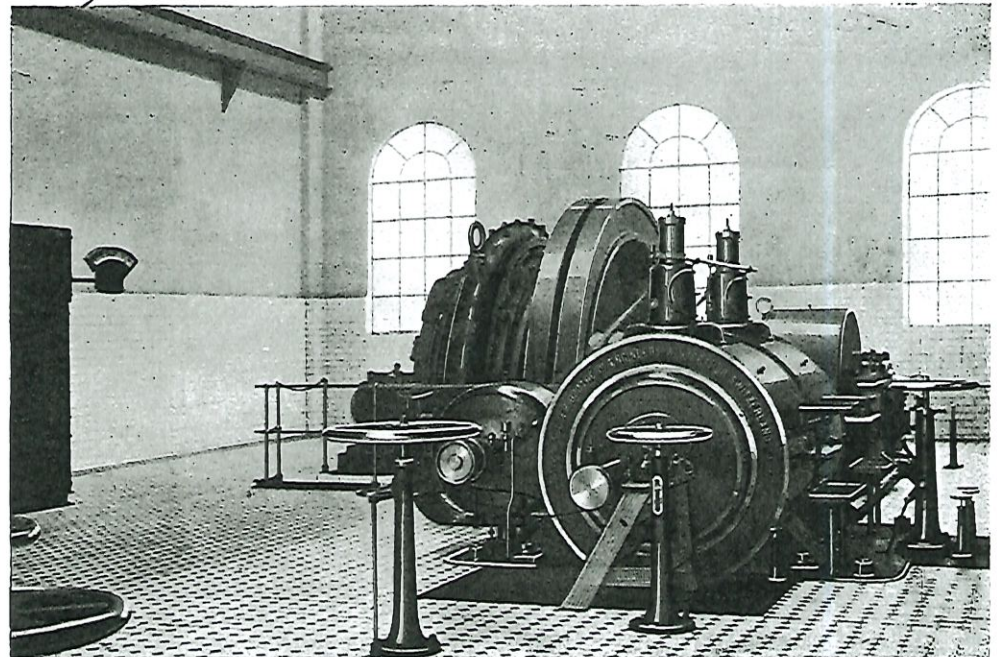
POWER PLANT. VIEW IN NO. 5 ENGINE HOUSE, SHOWING 800 K.W. GENERATOR.
