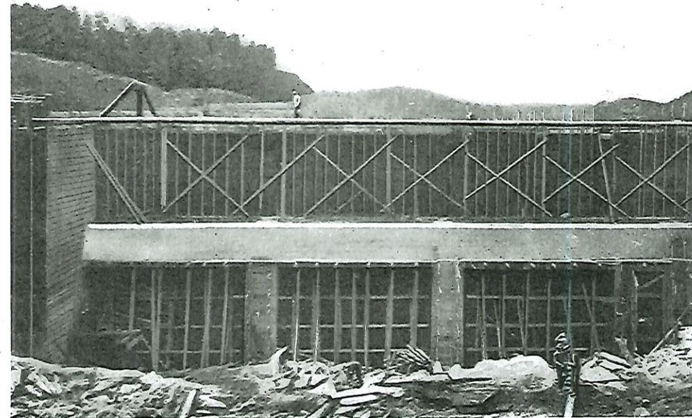
CONSTRUCTION OF NAIRN FALLS PLANT.—SEPTEMBER, 1915. SHOWING THREE MAIN UNIT INTAKES AND EXCITER INTAKE, AND PART OF THE BASEMENT WALL OF POWER HOUSE INTAKES. ON LEFT IS WING WALL. FORM WORK STILL IN PLACE.
