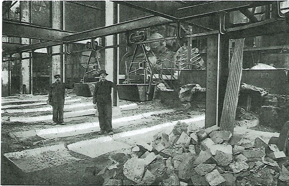
CONISTON PLANT. BESSEMER MATTE MOULDS IN SMELTER.
