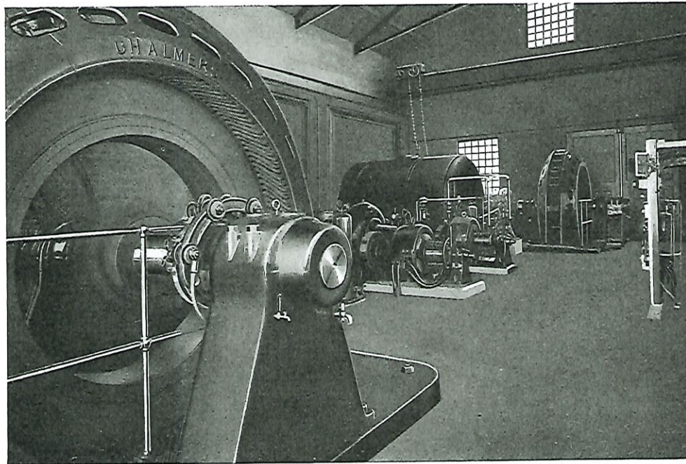
WABAGESHIK POWER PLANT. INTERIOR VIEW OF POWER HOUSE.
