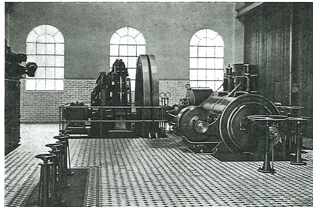
POWER PLANT. ANOTHER VIEW IN NO. 5 ENGINE HOUSE, SHOWING 800 K.W. GENERATOR.
