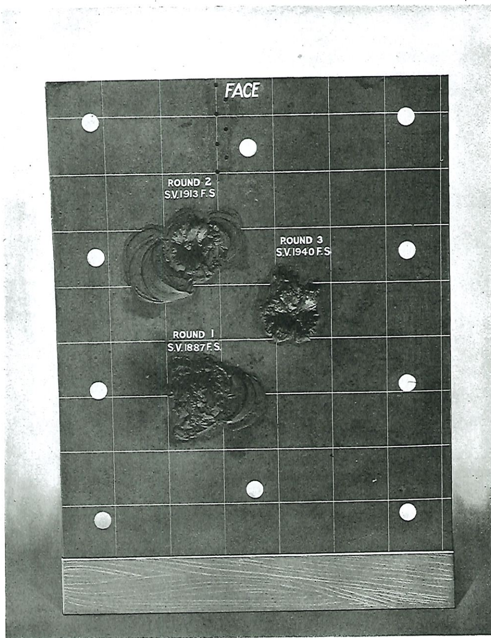
ARMOUR PLATE FOR BATTLESHIPS.
