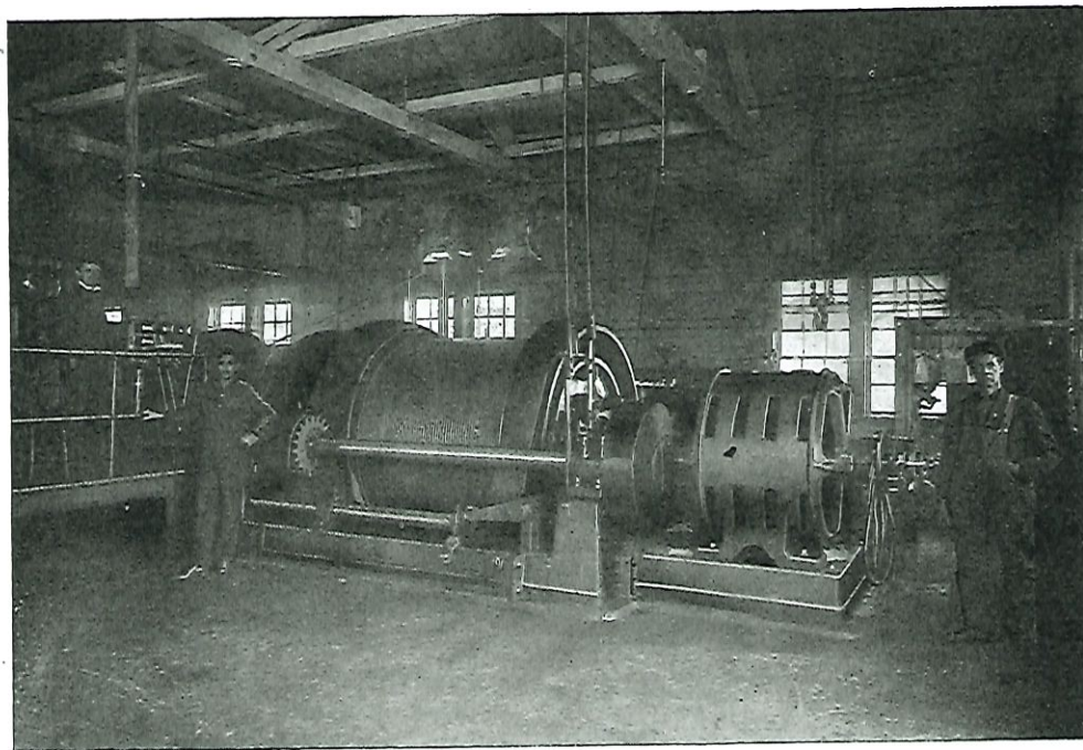
VICTORIA MINE. ELECTRICAL HOIST.
