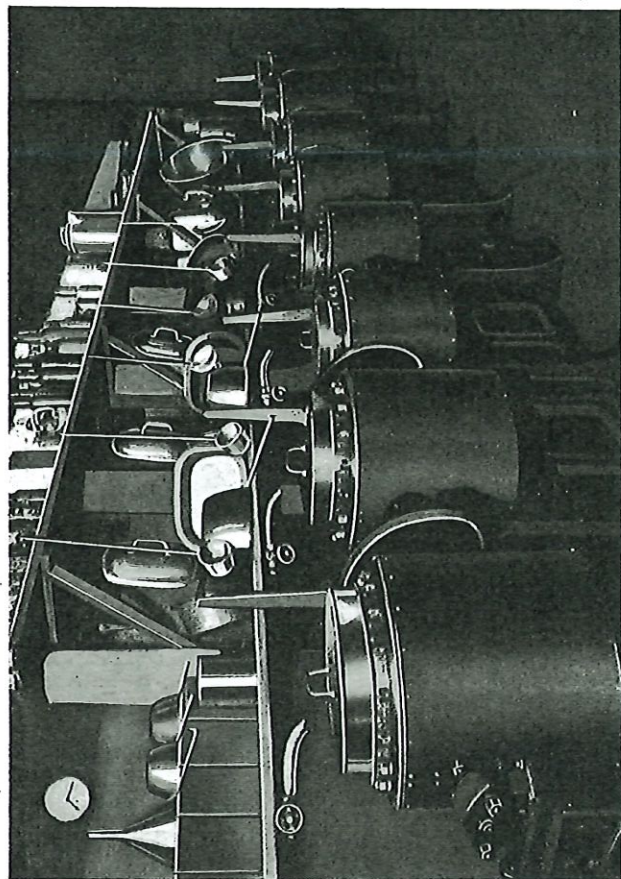
CRANSTON'S TEA ROOMS, LTD., GLASGOW. NICKEL-LINED STEAM JACKETS.
