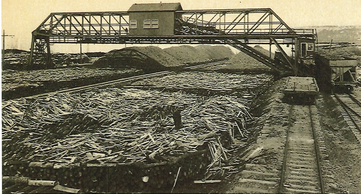
Green ore unloading bridge at O'Donnel roast yard.
