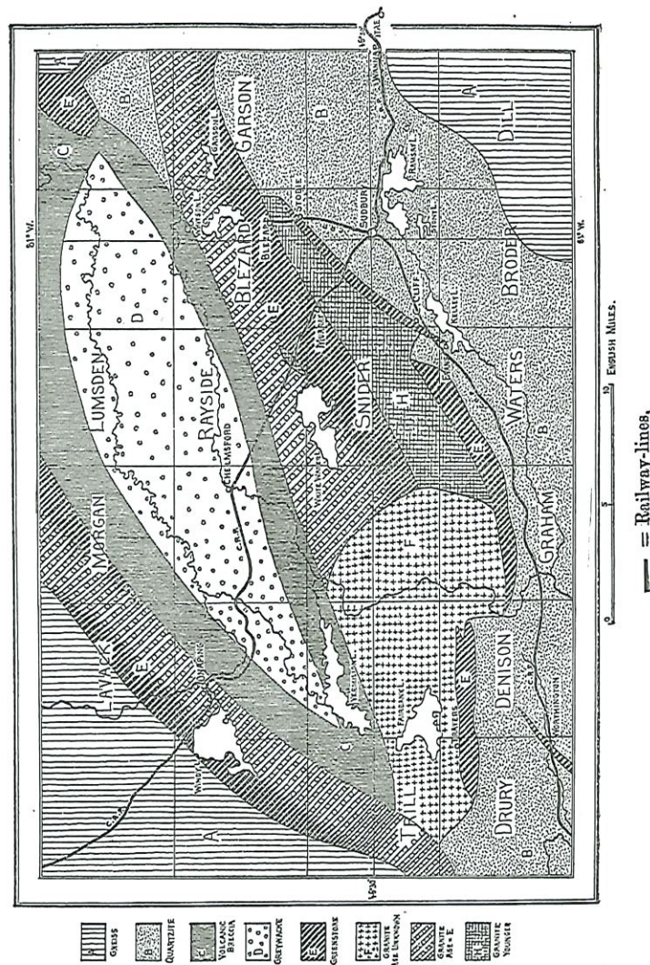
GEOLOGICAL SKETCH-MAP OF THE SUDBURY DISTRICT.
